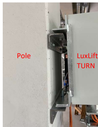
Suspension of LuxLift TURN
